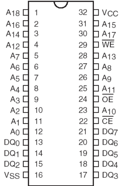
32-Pin DIP Module
